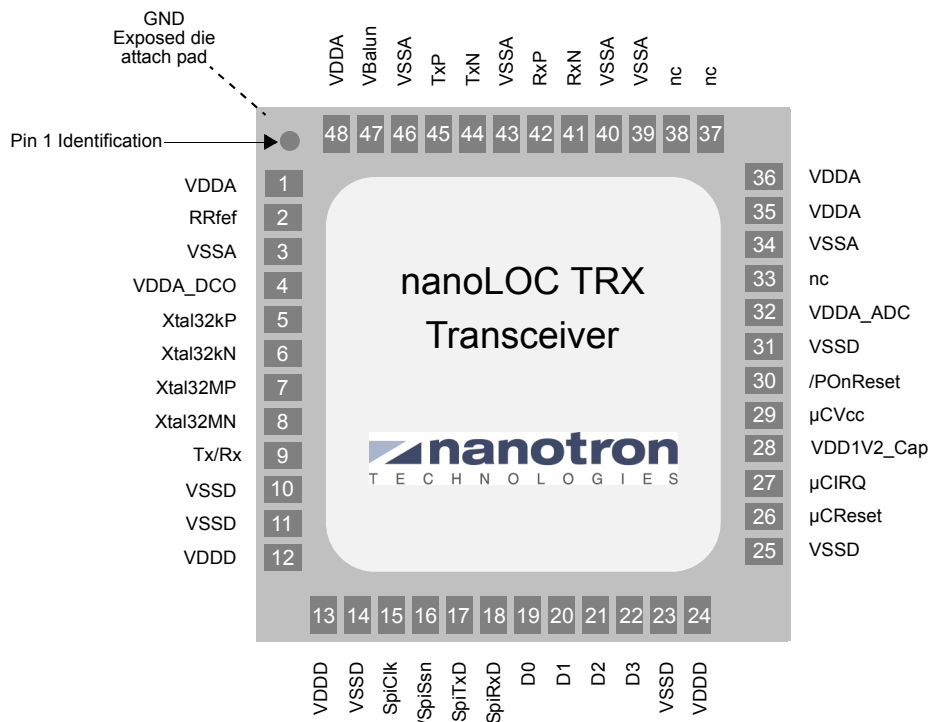
nanoLOC TRX Transceiver (NA5TR1) pin assignment (through top view)
