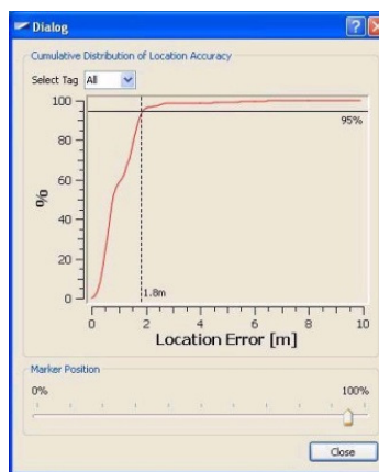
Cumulative Distribution Function
